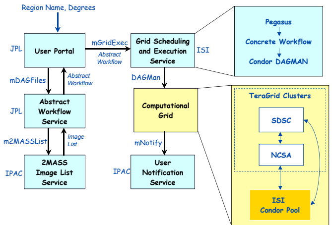
Fig. 2. The distributed architecture of the Montage TeraGrid Portal.
