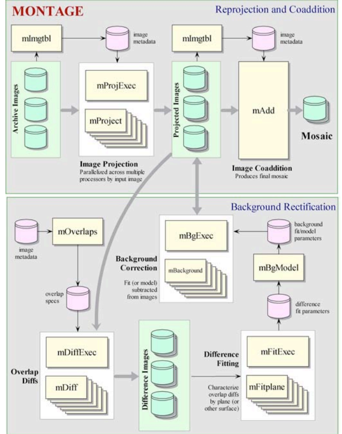
Fig. 1. The high-level design of Montage.
