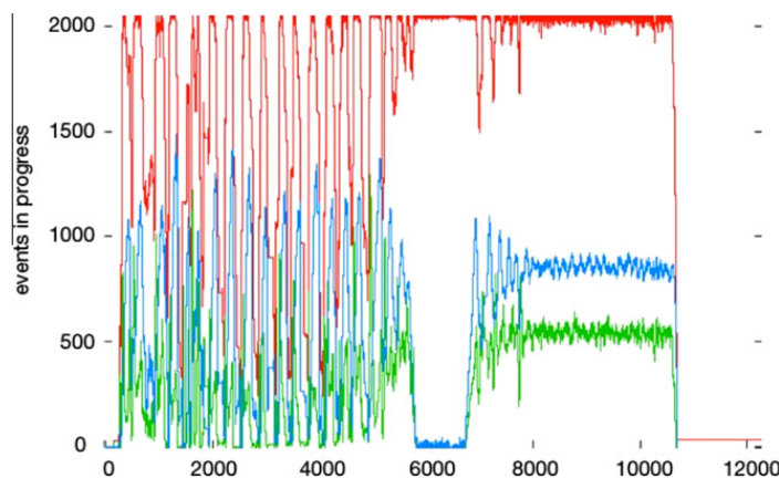
Fig. 3. 128 K-job SEM fMRI application execution on the Ranger Constellation (from [28]). Red = active compute jobs, blue = data stage in, green = stage out. (For interpretation of the references to color in this figure legend, the reader is referred to the web version of this article.)
