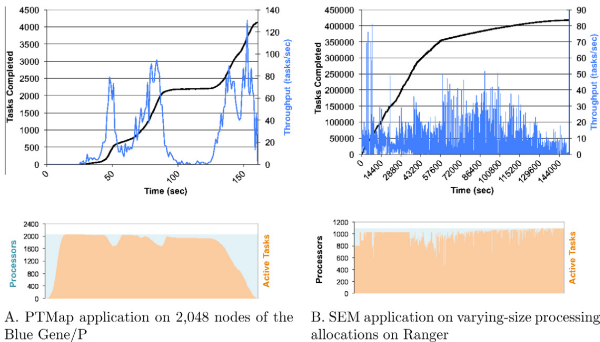
Fig. 4. Swift task rates for PTMap and SEM applications on the Blue Gene/P and Ranger (from [20]).
