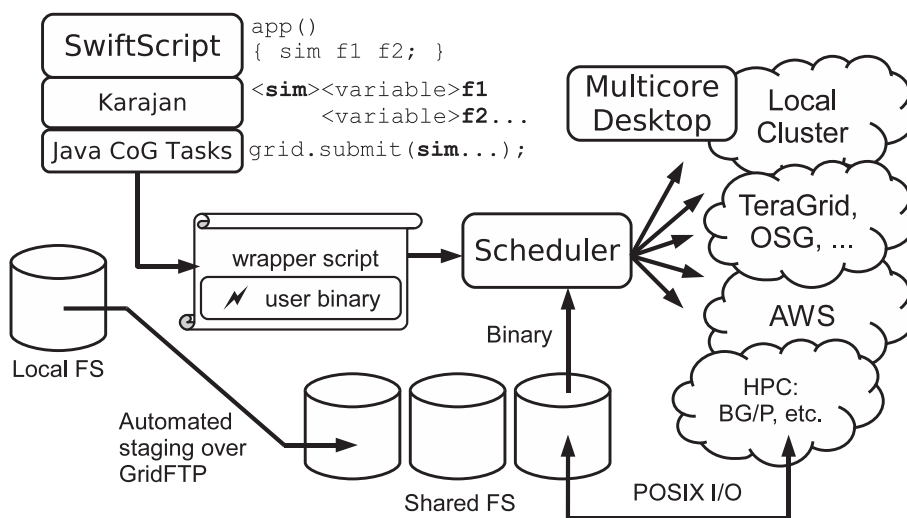
Fig. 1. Swift site model (CoG = Commodity Grid Java library [8], OSG = Open Science Grid, AWS = Amazon Web Services, HPC = high-performance computing system, BG/P = Blue Gene/P).
